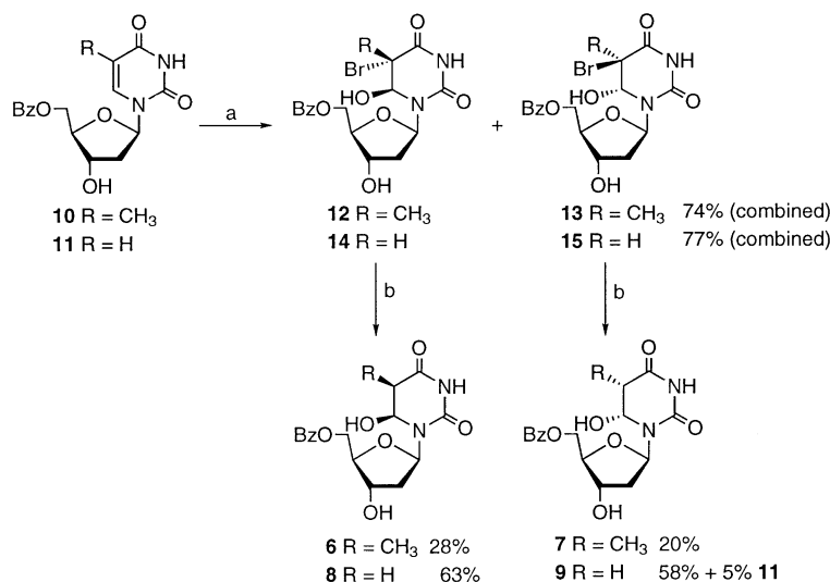
Scheme 1. (a) NBS, CaCO 3 , THF/H 2 O; (b) Zn/HOAc, THF/H 2 O.
