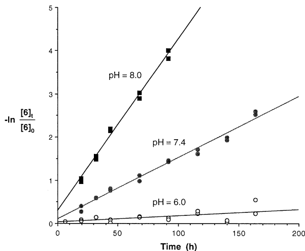
Figure 1. Disappearance of 6 as a function of time at 37 °C.
